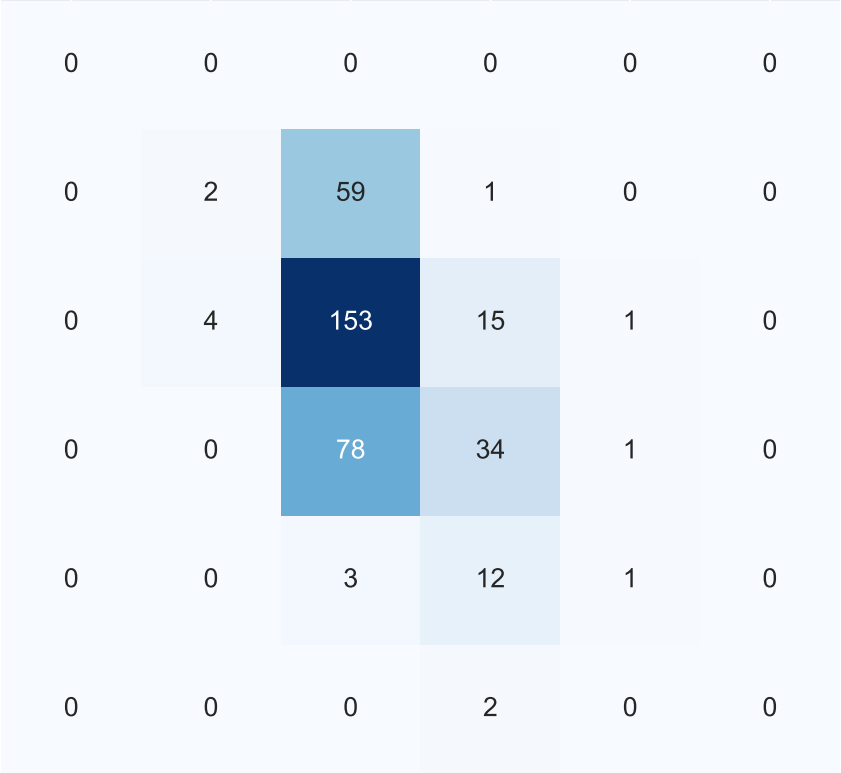
ARIMA (sinus) — test Exact: 51.9% ±1: 98.1% QWK: 0.360
